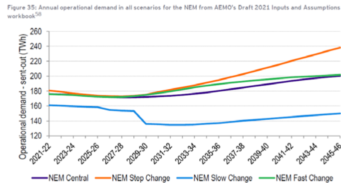
Figure 6 NEM demand (EY Figure 35)
