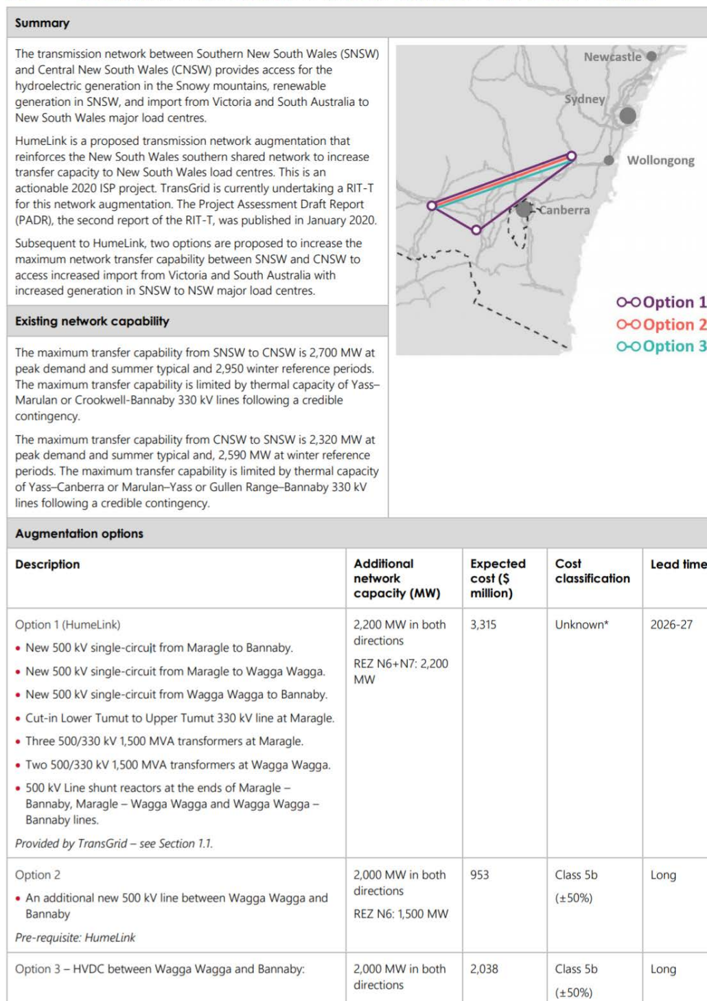
Figure 5 AEMO 2021 Transmission Cost Report (information from TransGrid)
